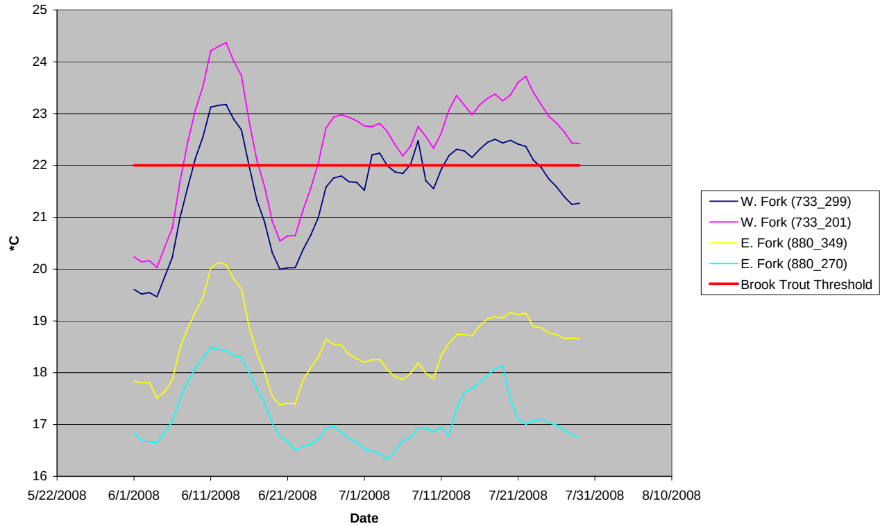
Rockymarsh Run East & West Fork 7 Day Max Avg.
