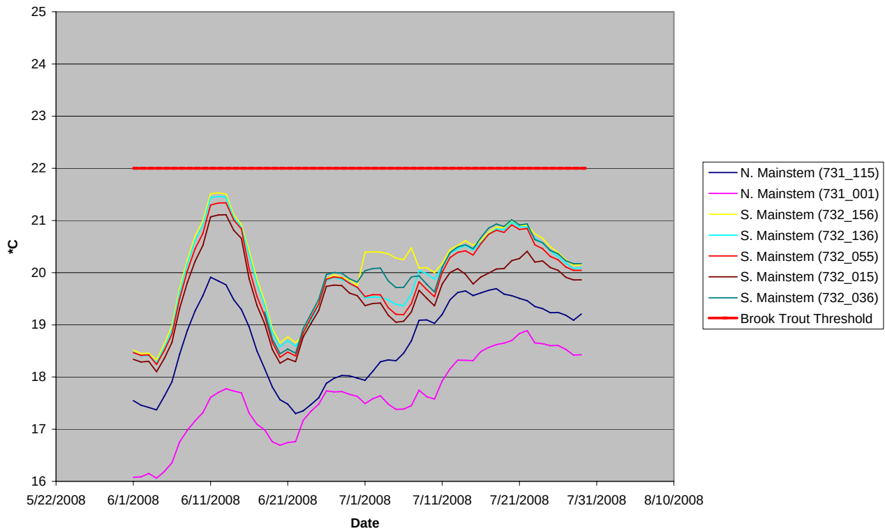
Rockymarsh Run Mainstem 7 Day Max Average
